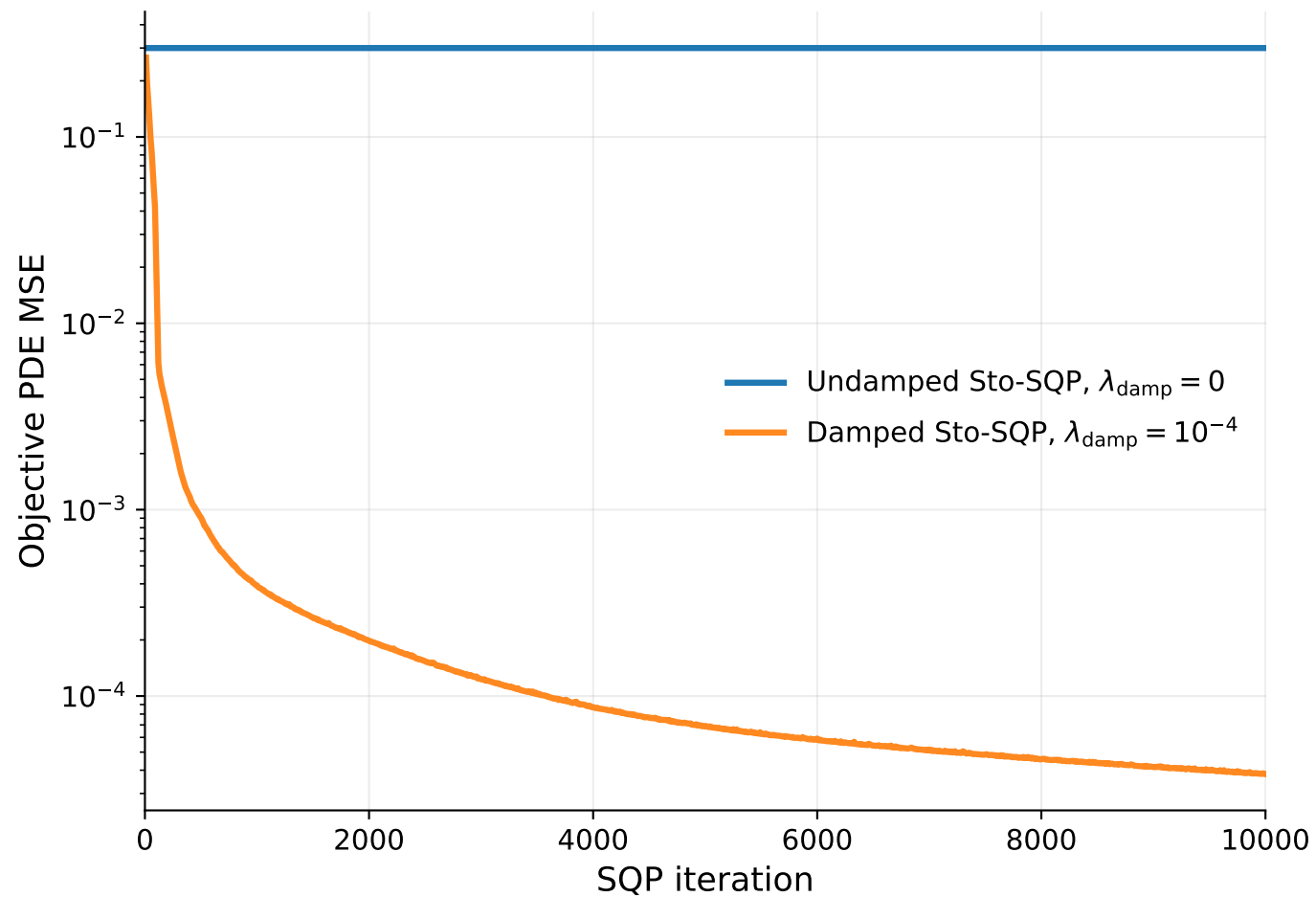
Burgers equation: objective PDE MSE
